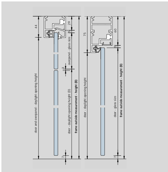
sectional cut
