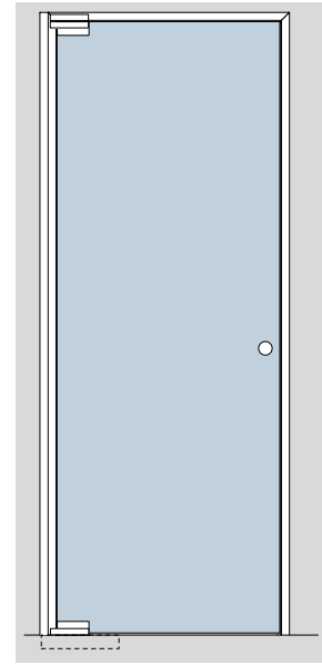
Type C Deubl AT 44 EA 3 sided frame profile with 1 sided accessory profile for floor closer (BTS).
