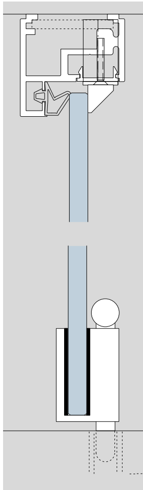
frame profile
