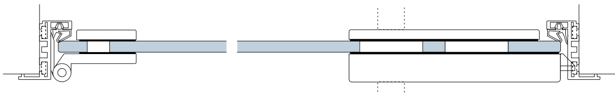
Deubl AT 23 E with DORMA special hinge Art. no. 11.294 resp. 12.050, lock Studio Rondo / Classic
