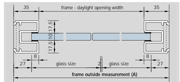
plan / fixed glazing with two elements
