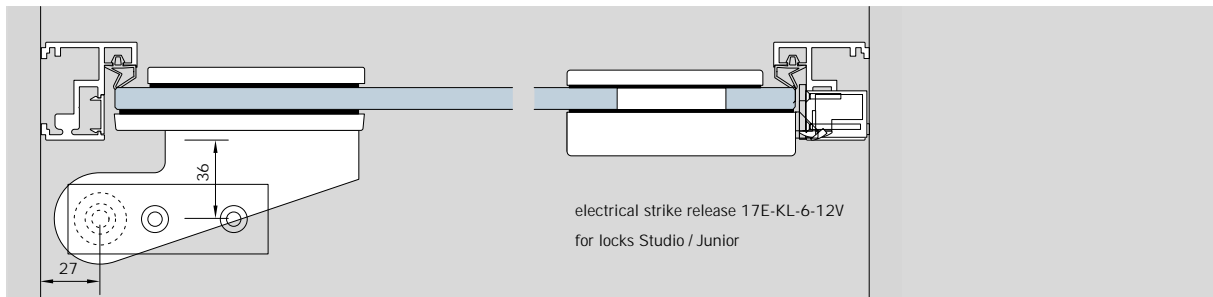
Deubl AT 44 with DORMA EA
