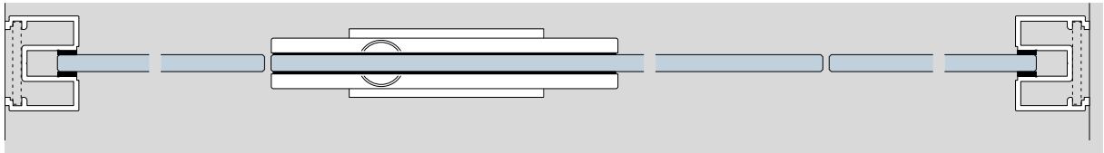
Deubl PT 35 with DORMA Universal patch fitting, floor pivot bearing
