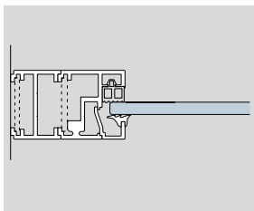
Deubl AT 44 fixed glazing with accessory profile
