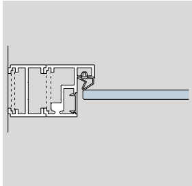
Deubl AT 44 with accessory profile
